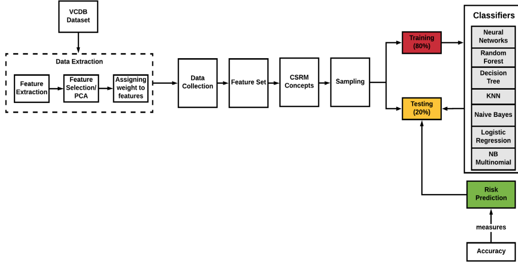
Figure 6: Classification process about the primary analysis
