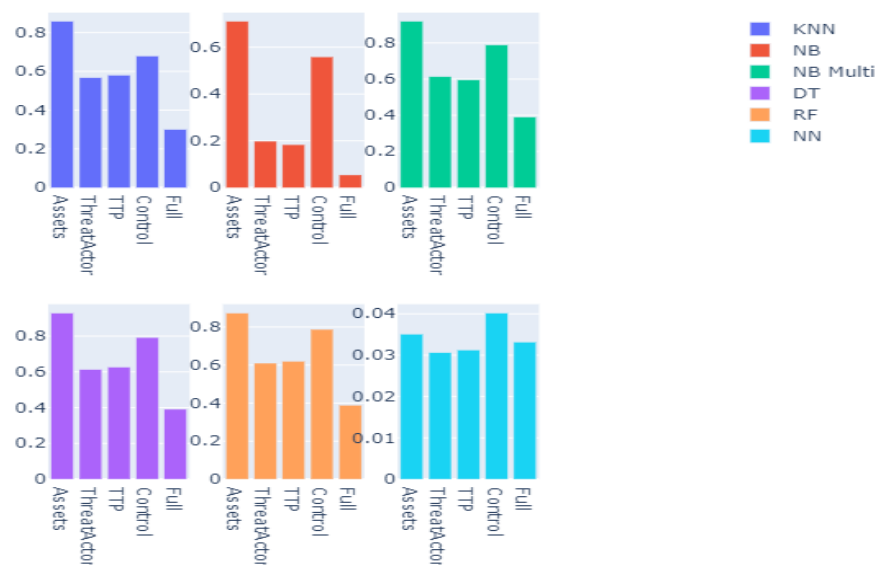
Figure 12. The accuracy of different classifiers for various types of input binary features
