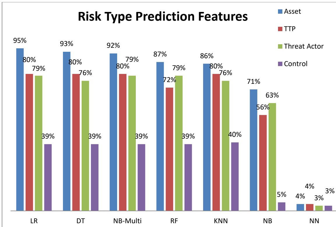
Figure 11: Performance of the features on each of the classifiers for predicting risk types
