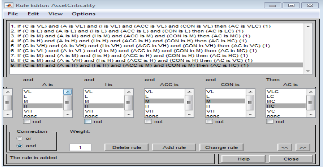
Figure 4: Rules Set for FACS
