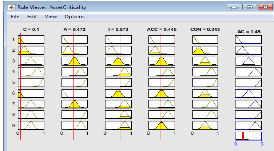
Figure 5: Sample of Rules
