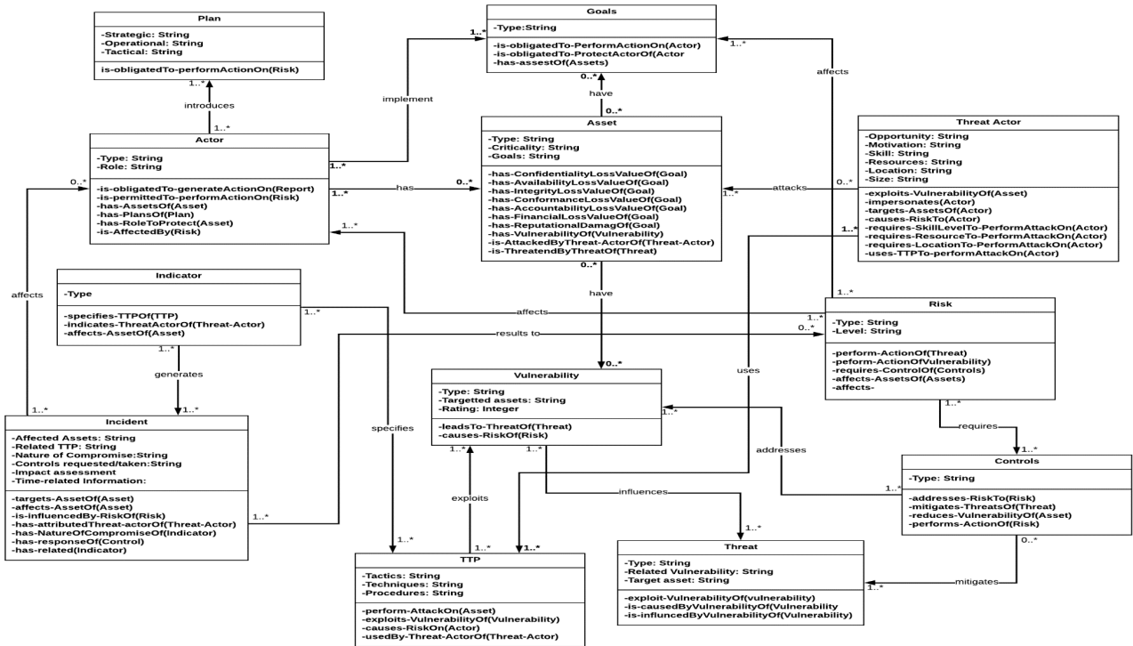
Figure 1: A meta-model for i-CSR at an organisational level
