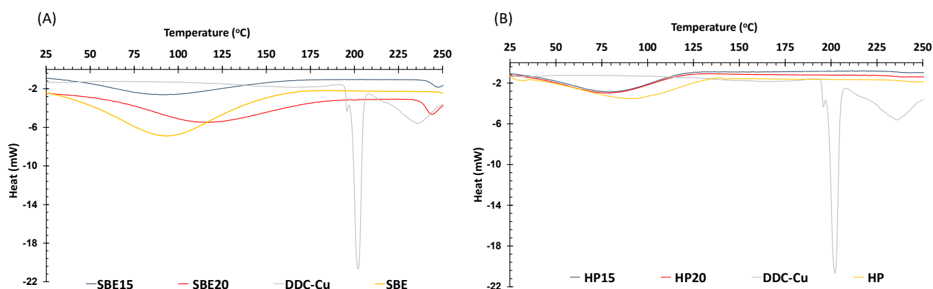
Figure 3. DSC thermographs of (A) SBE-CD freeze dried formulations, SBE-CD and DDC-Cu and (B) HP-CD freeze dried formulations, HP-CD and DDC-Cu.
